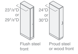
Locker
