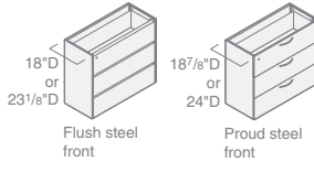
Drawer Stack
