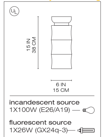
lantern cylinder ceiling
