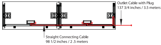
AV-Elec 2 Outlet Cable with Plug and Straight Connecting Cable
