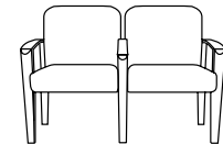
2600□-22, Two Seat with full intervening arm W=46", D=25", H=33¾" SH=18½", AH=25½"
