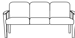
2600□-30, Three Seat W=64½", D=25", H=33¾" SH=18½", AH=25½"
