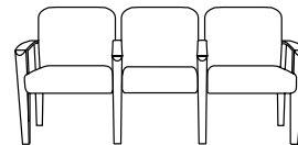
2600□-33, Three Seat with full intervening arms W=68", D=25", H=33¾" SH=18½", AH=25½"
