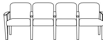
2600□-44, Four Seat with full intervening arms W=90", D=25", H=33¾" SH=18½", AH=25½"
