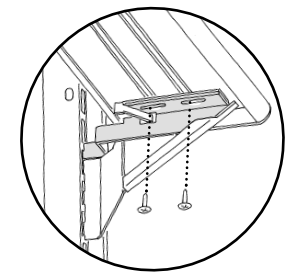
Detail of locking tab for Avenir and Series 9000 bracket. Lock bracket into panel, position assembled tray and attach with screws.
